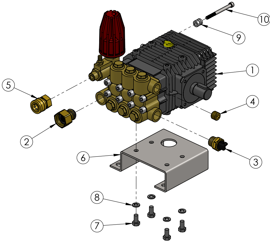
PUMP, 9.6WA15C SERVICE ASSEMBLY PART NO. 7104889
